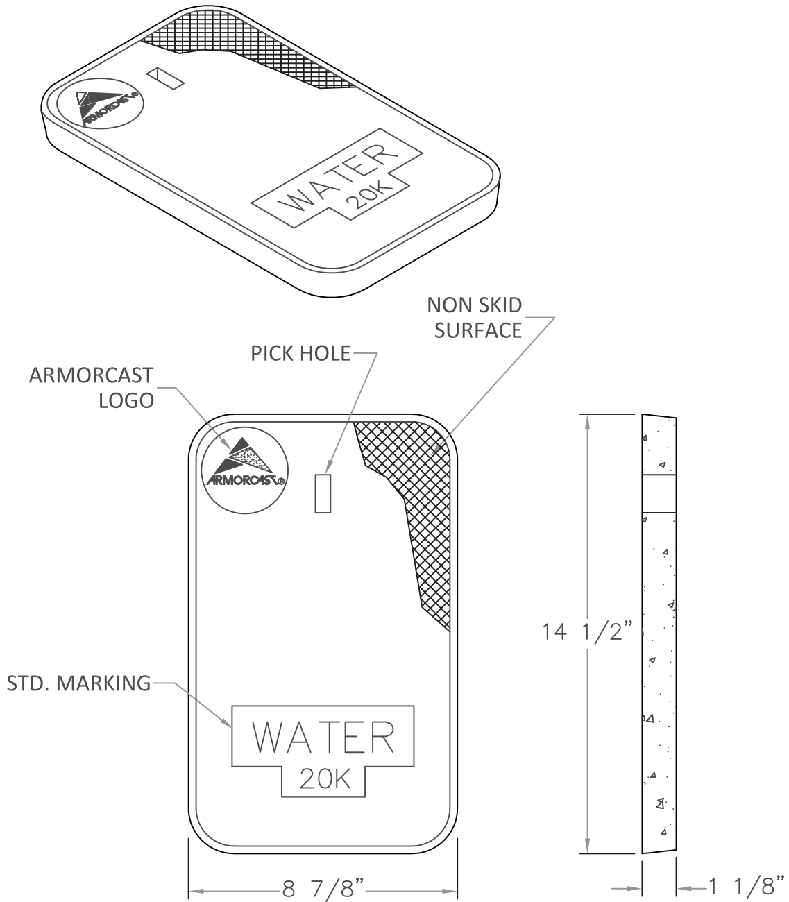
POLYMER CONCRETE LID ARMORCAST A6000482T
